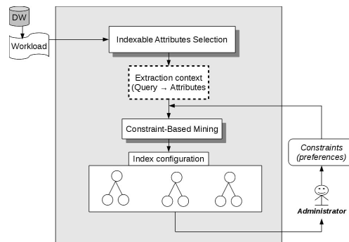
Figure 1: Constraint-based indexes selection.
