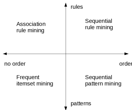
Figure 1 Sequential and non-sequential mining tasks
