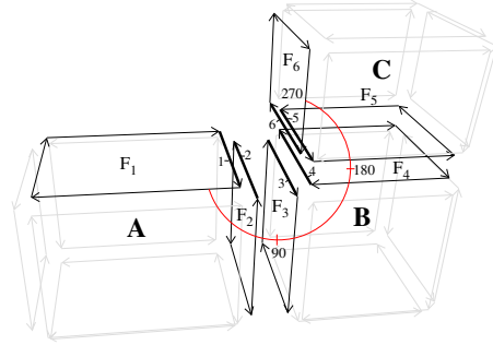
Figure 1: Combinatorial map representation of three volumes A , B and C . The six faces in dark lines share the same edge (described by the 6 darts drawn as bold arrows and numbered from 1 to 6). The figure illustrates the angular sorting method using dart 1 as reference. Face F_1 is linked by \beta_2 to face F_2 , face F_3 to F_4 , and face F_5 to F_6 .
