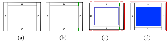
Figure 5: Face duplication process in 2D. (a) Four faces A, B, C and D. (b) Green edges symbolise common edges between two faces (2-sewn). (c) Unshared edges (not 2-sewn) are duplicated inside (blue edges) and outside (red edges). (d) Blue and red edges are 1-sewn to form the blue face (indoor volume in 3D) and the exterior envelop.
