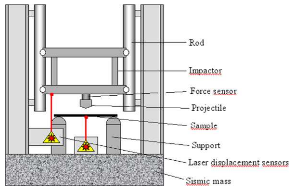
Fig. 2. Impact device.
