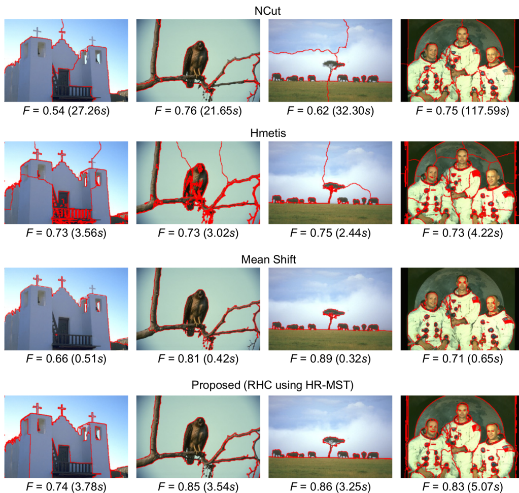
Fig. 12. Results of segmentations of images from the BSDB obtained with NCut [18], Hmetis [42], Mean Shift [39] and our proposed algorithm (using HR-MST). F -scores and computation times are displayed for each result.
