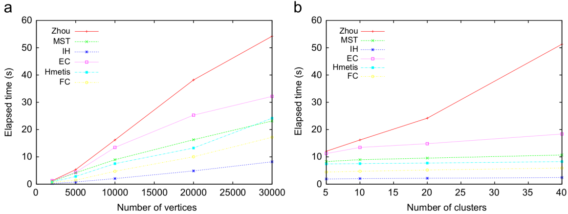
Fig. 11. Computation times for different clustering algorithms according to (a) the number of vertices N in the hypergraphs ( \lambda_t = 0.2 , k = 10 ) and (b) the number of clusters k ( \lambda_t = 0.2 , N = 10\,000 ).
