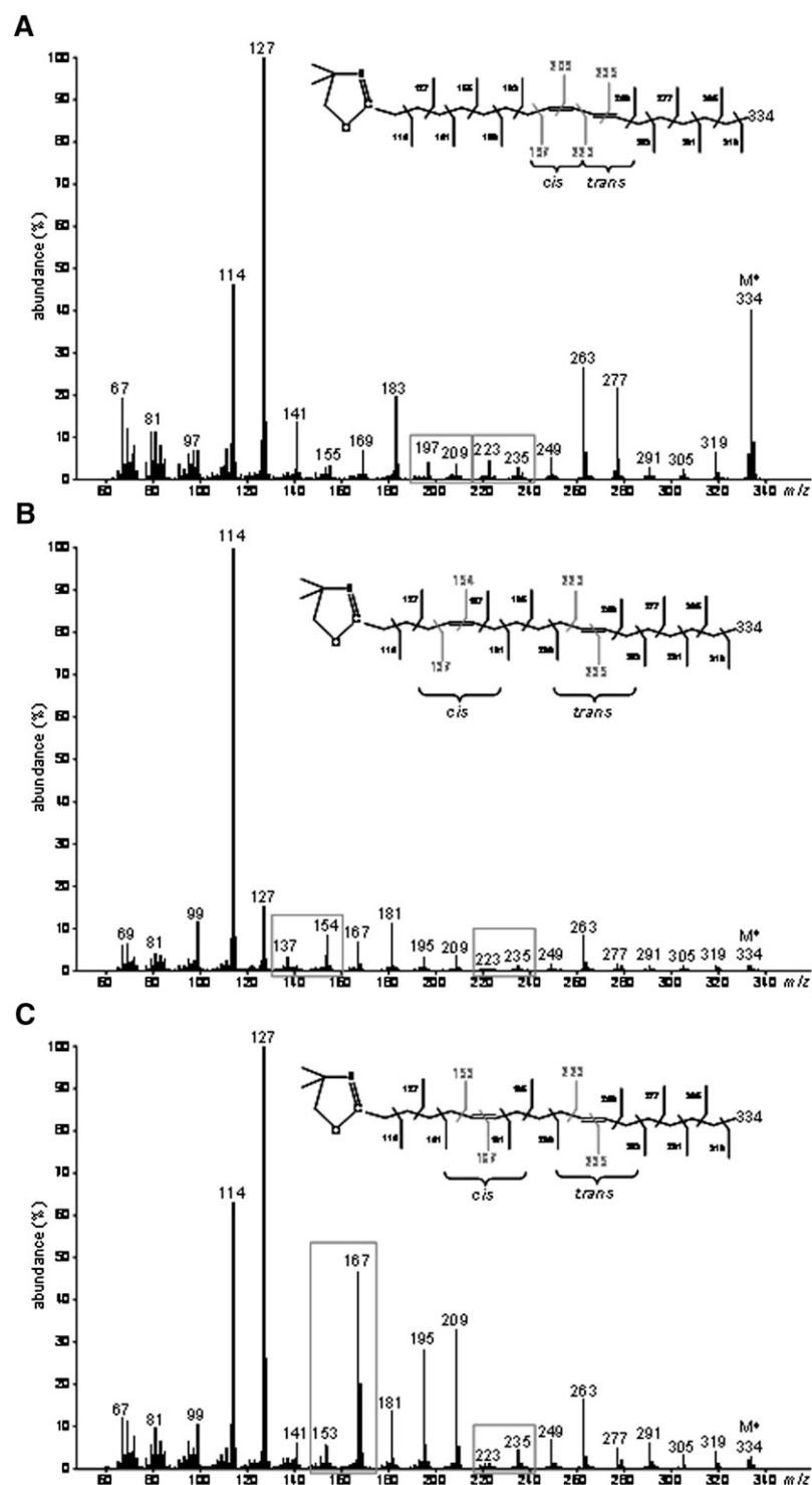
Fig. 5. Electron-impact mass spectra of DMOX derivatives of the different ^{13}\text{C} -octadecadienoic acids obtained after incubation of [ 1-^{13}\text{C} ]TVA with COS-7 cells expressing either rat FADS1 or FADS2. Molecular ions ( M^+ ) are m/z 334. (A) ^{13}\text{C} -rumenic acid ( R_t = 27.5 min) obtained after incubation of [ 1-^{13}\text{C} ]TVA with COS-7 cells in all the experimental conditions. (B) Unknown ^{13}\text{C} -octadecadienoic acid ( R_t = 21.9 min) obtained after incubation of [ 1-^{13}\text{C} ]TVA with COS-7 cells expressing rat FADS1. A gap of 12 amu was shown between ions containing 10 and 11 carbons ( m/z 223 and 235 amu) locating this double bond in position 11-12, while the ion at m/z 154 amu was a diagnostic guide for a double bond in position 5-6 (59). This fatty acid was therefore identified as \Delta 5,11-18:2 ( cis 5, trans 11-18:2) (C) Unknown ^{13}\text{C} -octadecadienoic acid ( R_t = 22.1 min) obtained after incubation of [ 1-^{13}\text{C} ]TVA with COS-7 cells expressing rat FADS2. A gap of 12 amu was shown between ions containing 10 and 11 carbons ( m/z 223 and 235 amu) locating this double bond in position 11-12, while the fingerprint ions at m/z 153, 167, and 181 amu identified a double bond in position 6-7 (60). This fatty acid was therefore identified as \Delta 6,11-18:2 ( cis 6, trans 11-18:2). Representative example of n = 3 distinct experiments.
