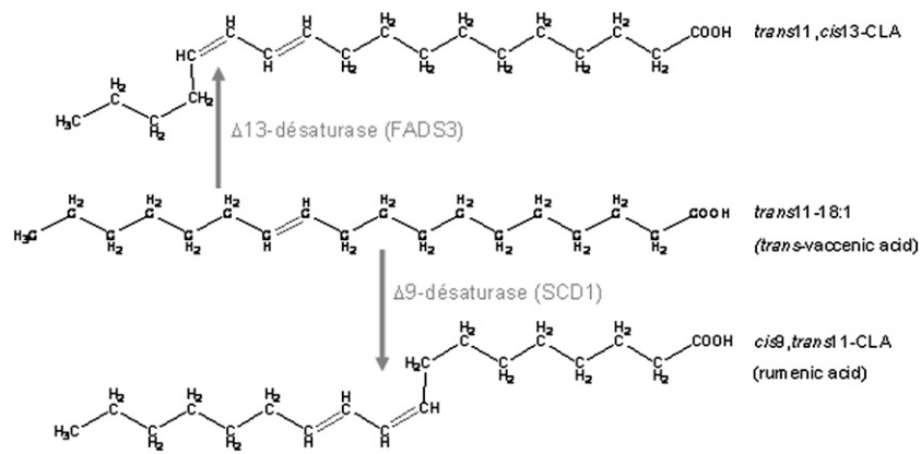
Fig. 11. Proposed metabolic pathway of trans -vaccenate conversion into cis 9 , trans 11 -CLA catalyzed by the Δ9-desaturase and into trans 11 , cis 13 -CLA by the newly discovered FADS3-catalyzed Δ13-desaturase.
