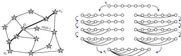
Figure 2: Left : The graph-of-graph \mathcal{G} connects named networks (represented as stars). Two networks are neighboring iff they differ by a graph edit distance of one. The centrality distance defines a distance for each pair of neighboring graphs. Right : Two possible evolutionary paths from a line graph G_1 to a shell graph G_2 .
