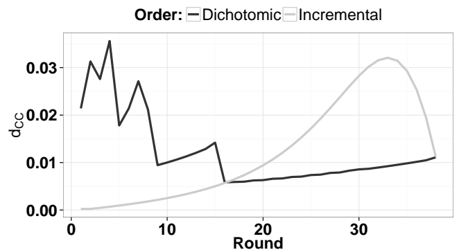
Figure 3: Evolution of closeness centrality distance d_{CC} from G_L to G_S for n = 40 . Dichotomic and incremental paths are depicted in Figure 2 ( right ). Both order define a different path in \mathcal{G} from G_L to G_S . At each step, the closeness centrality-induced distance between G_i and G_{i-1} is computed.
