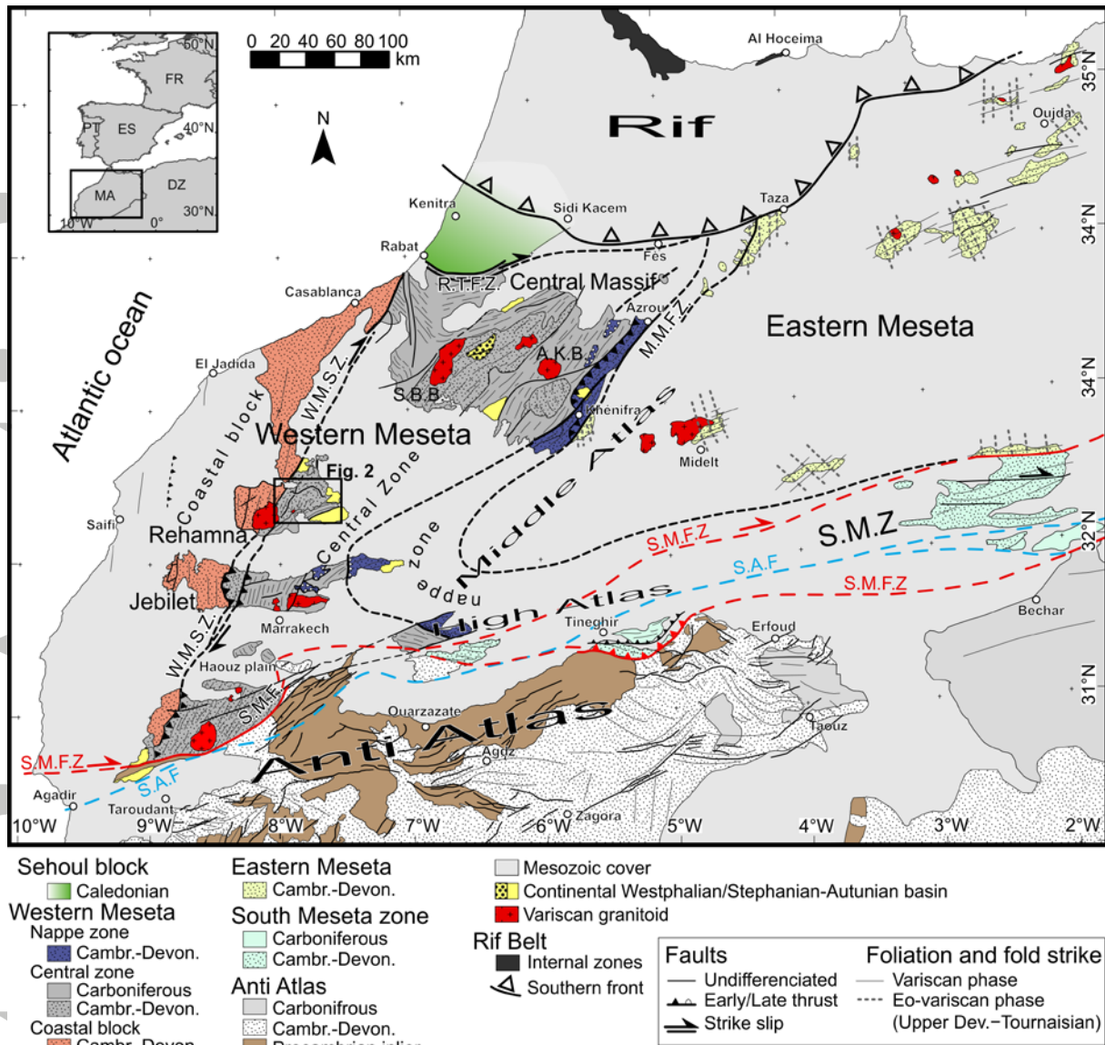
Figure 1. Simplified geological map of the Moroccan Variscides [Modified after Hæpffner et al. , 2005; Michard et al. , 2008 and Michard et al. , 2010b]. Middle Meseta Fault Zone (M.M.F.Z.), Western Meseta Shear Zone (W.M.S.Z.), South Meseta Fault Zone (S.M.F.Z.), South Atlas Fault (S.A.F.), Rabat-Tiflet Fault Zone (R.T.F.Z.), Sidi Bettache basin (S.B.B.), Azrou Khenifra basin (A.K.B.).
