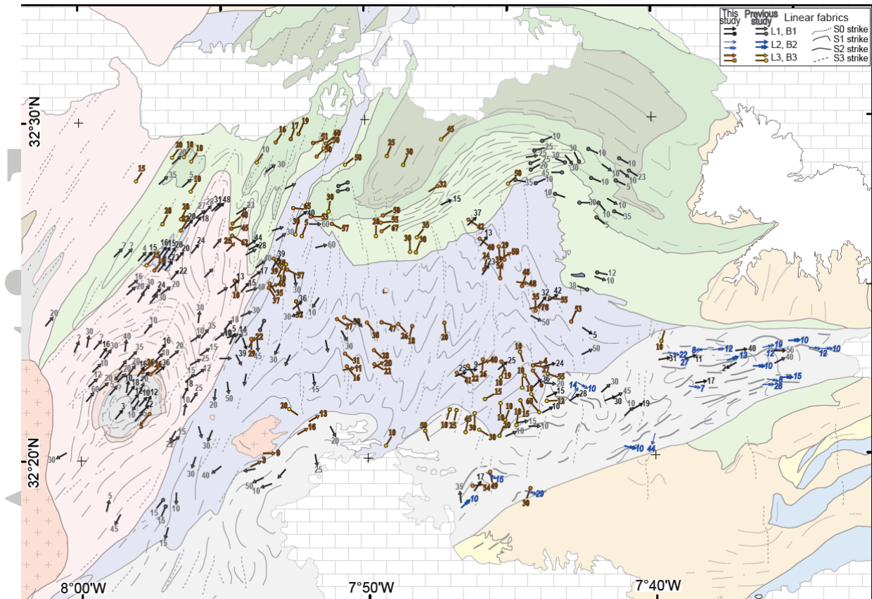
Figure 7. Structural map of linear structures with the trend of planar structures from Figure 6 including data from this study and from Hæpffner [1974]; Cornée [1982]; Lagarde and Michard [1986]; Corsini [1988]; Corsini et al. [1988b]; Diot [1989]; Aghzer and Arenas [1995]; Baudin et al. [2003] and Razin et al. [2003].
