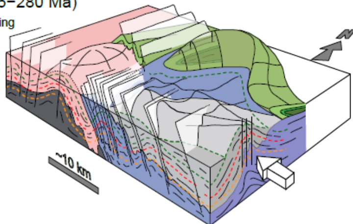
Figure 10. 3D idealized model for the evolution of the Rehamna massif (see text for discussion).
