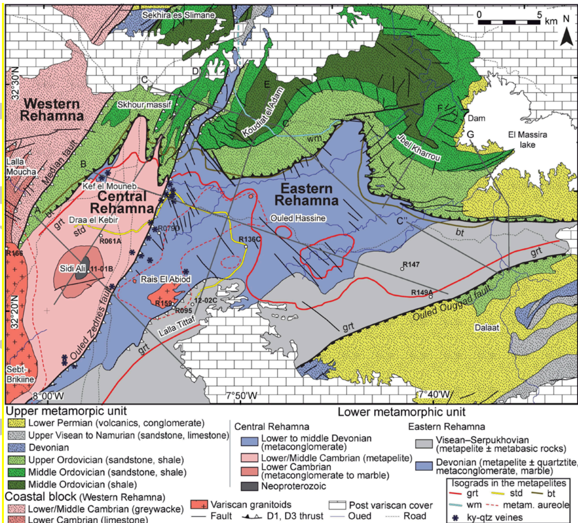
Figure 2. Lithological map of the Rehamna massif [modified after Hæpffner et al. , 1975b; Michard, 1982; Cornée, 1982; Corsini, 1988; Corsini et al. , 1988b; Baudin et al. , 2003; Razin et al. , 2003; El Kamel and El Hassani, 2006 and Michard et al. , 2010] showing the locations of samples used for geochronology. Grt and Bt isograds modified after Michard [1982]; Cornée and Muller [1981]; Cornée [1982]; Baudin et al. [2003]; Razin et al. [2003]; St isograd modified after Hæpffner et al. [1982] and Aghzer and Arenas [1995].
