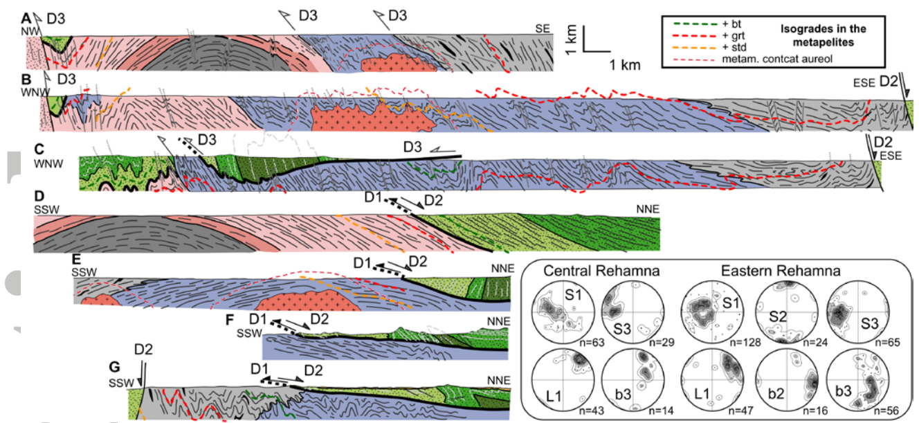
Figure 4. Interpretative geological cross sections through the Rehamna massif. Stereographic diagrams show equal-area, lower-hemisphere projections of planar and linear structures.
