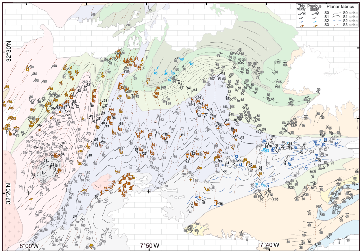
Figure 6. Structural map of planar structures in the Rehamna showing the distribution and relationships between planar fabrics with data from this study and from Hoepffner [1974], Cornée [1982], Lagarde and Michard [1986], Corsini [1988], Corsini et al. [1988a], Diot [1989], Aghzler and Arenas [1995], Baudin et al. [2003], and Razin et al. [2003].
