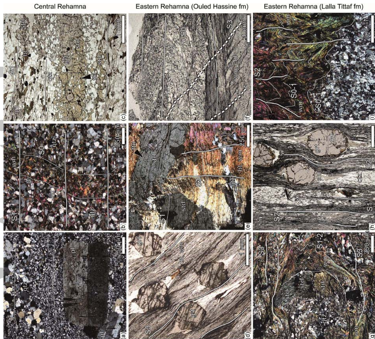
Figure 8. Photomicrographs illustrating the relationships between metamorphic minerals and microstructures in the lower metamorphic unit. (a) Development of the S1 metamorphic foliation in the Lower Cambrian metagreywacke from the Sidi Ali dome. (b) S0 layering reworked by recumbent open F1 fold in Devonian metapelite from Kel El Mound. (c) Staurolite with garnet inclusions parallel to the S1 metamorphic foliation in micaschist from Lower/Middle Cambrian rocks north of the Sidi Ali dome. (d) Intense shearing around garnet porphyroblast in mica schist from the Ouled Zednes fault zone. (e) Staurolite bearing mica schist with S1 foliation weakly affected by F3 asymmetric folds (Ouled Hassine formation). (f) F1 folds slightly reworked by asymmetric F3 folds in a biotite-bearing mica schist from
