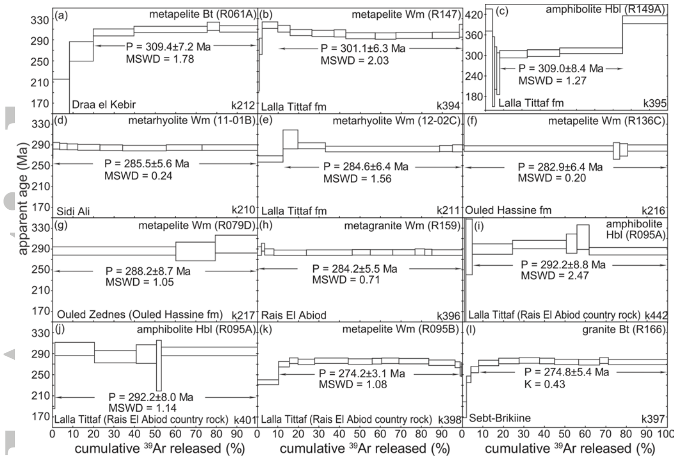
Figure 9. ^{40}\text{Ar}/^{39}\text{Ar} age spectra as a function of released ^{39}\text{Ar} on white mica (Ms), Biotite (Bt) and hornblende (Hbl) single grains of samples from the infrastructure. Rock type and analysed mineral are given together with the sample number (in brackets) and the analytical reference of the laboratory (bottom right hand side; see Tables A1–A12 for raw data). The error boxes for each step and for the flat spectrum part ages are at the 2\sigma level. Ages were calculated using the ArArCalc program of Koppers [2002].
