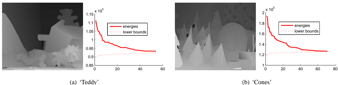
Fig. 13: Stereo matching results for ‘Teddy’ (a) and ‘Cones’ (b) when using a higher-order discontinuity preserving smoothness prior. We show plots for the corresponding sequences of upper and lower bounds generated during the primal-dual method. Notice that these sequences converge to the same limit, meaning that the estimated solution converges to the optimal value.
