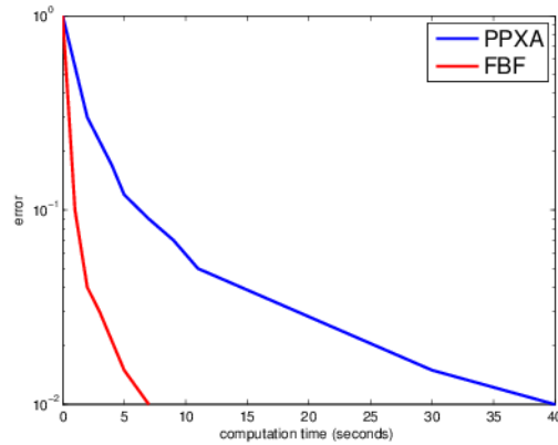
Fig. 7: Comparison of the convergence speed of a Douglas-Rachford based algorithm (PPXA [65]) (blue) and an FBF-based primal-dual algorithm (red) for image denoising using a non-regular graph, Matlab implementation on an Intel Xeon 2.5GHz 8-core system.
