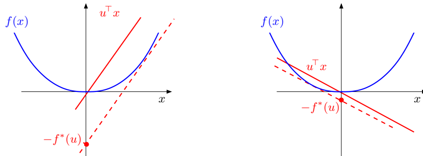
Fig. 4: Graphical interpretation of the conjugate function.
