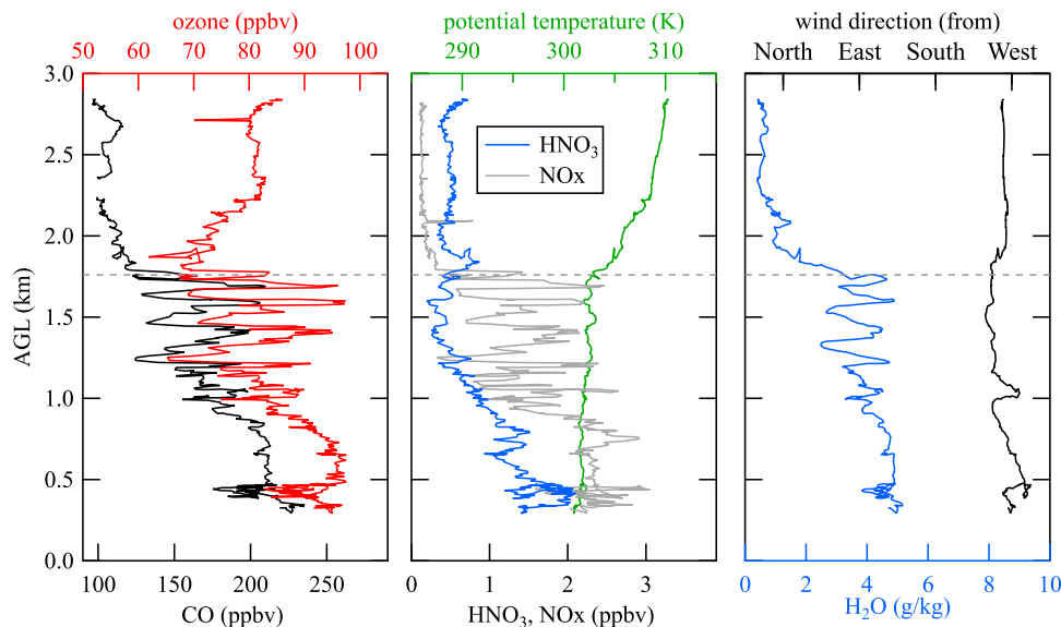
Figure 4. One-second ozone (red), CO (black), HNO 3 (blue), and NO x (gray) measurements and meteorological observations (potential temperature in green, wind direction in black, and water vapor in blue) during a spiral ascent over Redlands, CA at 3:20 P.M. PDT on 8 May 2010. The gray dashed line indicates the boundary layer height.
