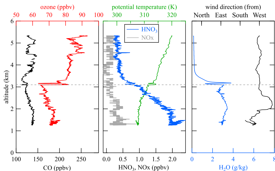
Figure 12. Same as Figure 4 but for a profile over Joshua Tree NP at 3:15 P.M. PDT on 4 May 2010. Since CLD instrument diagnostics were performed during this ascent, NO x data from the cavity ring-down spectrometer are shown.
