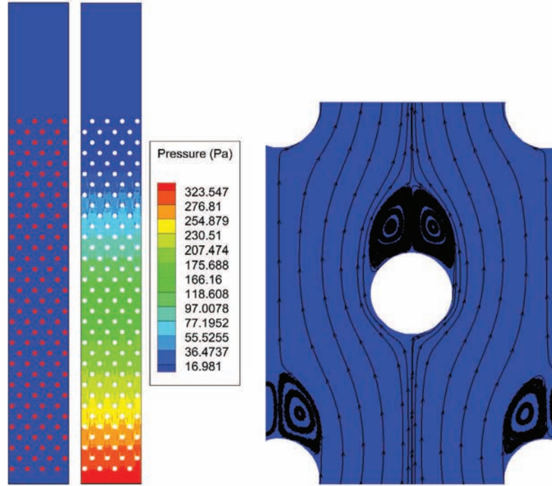
Fig. 21. Two-dimensional flow across a fixed array of cylinders – the positions of the cylinders in the tank (left), the macroscopic pressure across the fixed bed (middle), and a zoom on the velocity field in the vicinity of a particle (right) are presented.
