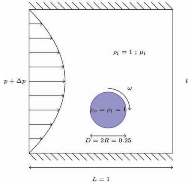
Fig. 18. Definition sketch of the Poiseuille flow corresponding to the first configuration of [100].
