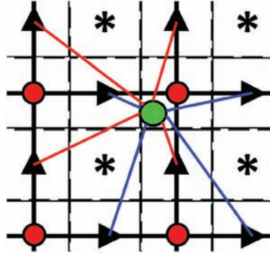
Fig. 4. Eulerian velocity kernel (u-components in blue and v-components in red) used in two dimensions to estimate the components of the interpolation Lagrangian velocity points (green point). (For interpretation of the references to color in this figure, the reader is referred to the web version of this article.)
