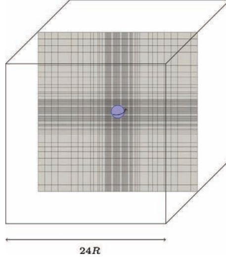
Fig. 14. Typical Eulerian grid used to simulate the rotation of a particle in a box with N_d = 20 .
