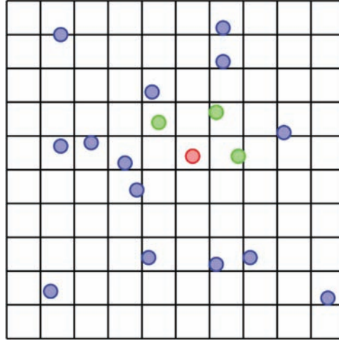
Fig. 7. Searching of particle collision inside a CPU box distribution of 10 \times 10 in two dimensions – the red particle is detected to interact with green particles whereas no interaction is considered with the blue ones. (For interpretation of the references to color in this figure, the reader is referred to the web version of this article.)
