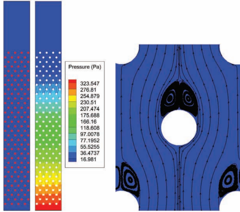
Fig. 21. Two-dimensional flow across a fixed array of cylinders – the positions of the cylinders in the tank (left), the macroscopic pressure across the fixed bed (middle), and a zoom on the velocity field in the vicinity of a particle (right) are presented.
