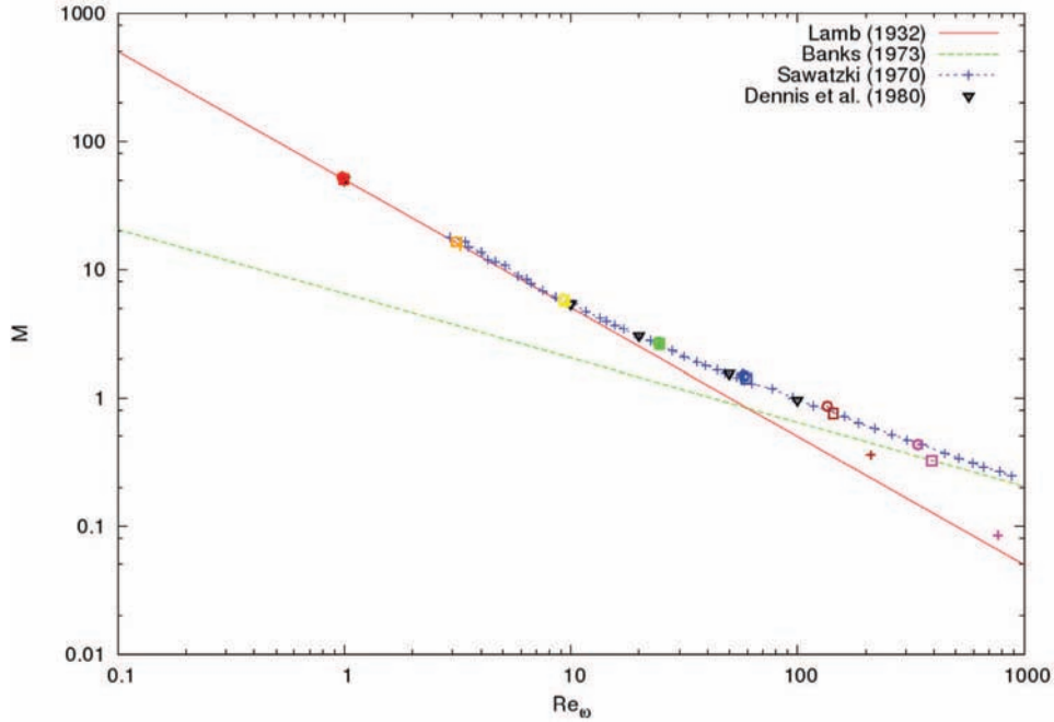
Fig. 17. Relation between the Reynolds number and the dimensionless torque. Lines correspond to references cited below. Symbols correspond to actual for different refinements (cross, circle and square for 10, 20 and 40 nodes per diameter). Colors (red, orange, yellow, green, blue, magenta and pink) are respectively for \mu = 10^b , b = \{0, 0.5, \dots, 3\} . (For interpretation of the references to color in this figure, the reader is referred to the web version of this article.)
