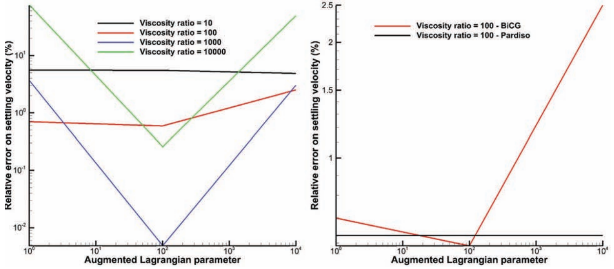
Fig. 10. Comparison of relative errors on settling velocity: left, results obtained with the iterative solver for various viscosity ratios and augmented Lagrangian parameter \mathcal{K} and right, comparison of PARDISO and BiCGSTAB II for a viscosity ratio of 100.
