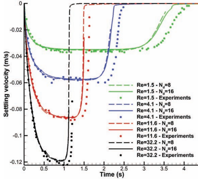
Fig. 13. Settling velocity over time for the test case of [82] – long dashed line is associated to N_d = 8 , straight line to N_d = 16 and symbols to experiments [82]. Green, blue, red and black colors are related respectively to Re = 1.5 , Re = 4.1 , Re = 11.6 and Re = 32.2 . (For interpretation of the references to color in this figure, the reader is referred to the web version of this article.)
