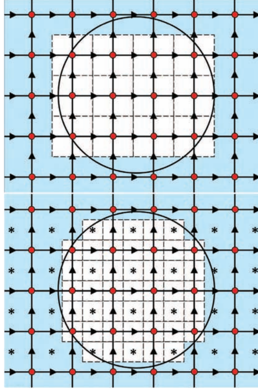
Fig. 2. Discrete interpretation of the direct viscous penalty method (top) and split viscous penalty approach (bottom) on staggered grids – the pressure points are plotted in red circles, the velocities as arrows and the pure shearing and rotations viscosities as stars. The black line represents the interface between a particle and the carrier fluid.
