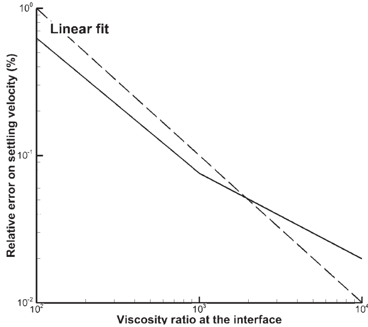
Fig. 11. Sensitivity of the relative error on U_\infty obtained with the PARDISO solver for various viscosity ratios.
