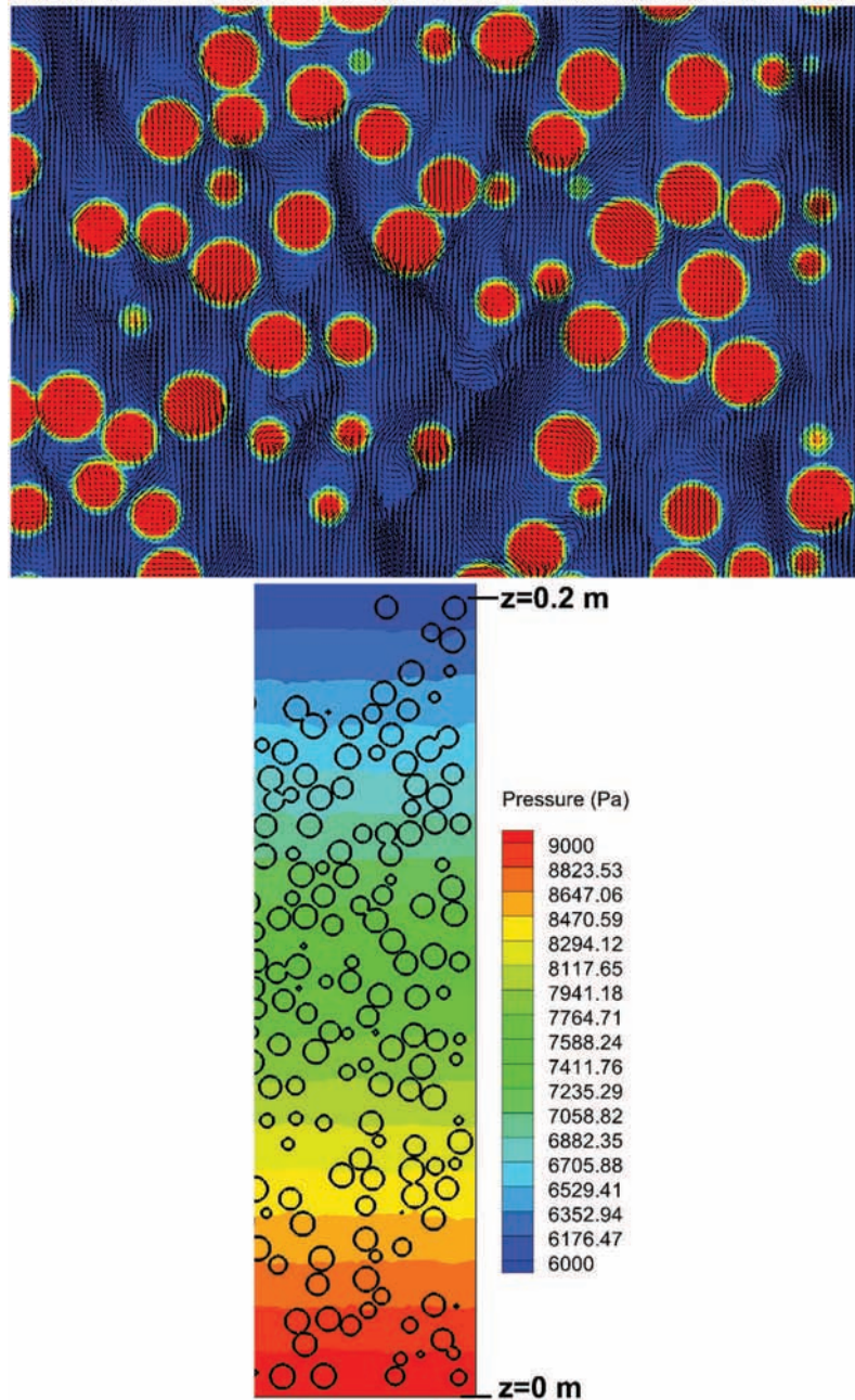
Fig. 24. Instantaneous view of the fluidized bed in a medium vertical slice at t = 10 s – top: particles and velocity field in a zoom – bottom: particles (lines) and pressure in the whole bed. (For interpretation of the references to color in this figure, the reader is referred to the web version of this article.)
