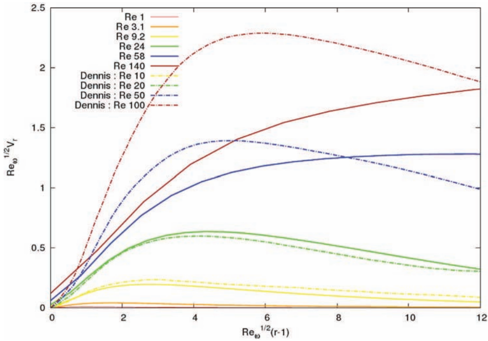
Fig. 16. Radial velocity at the meridian.
