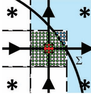
Fig. 5. Two-dimensional network of 10^{Nd_{dim}} virtual points used to estimate the local solid fraction C^{n+1} thanks to a Lagrangian position \mathbf{X}^{i,L,n+1} of a particle, whose interface is noted \Sigma . In green are plotted the virtual points belonging to the particle and in blue the other ones. In the example, C^{n+1} = 92/100 = 0.92 . (For interpretation of the references to color in this figure, the reader is referred to the web version of this article.)
