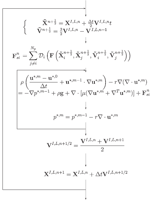
Fig. 8. Work-flow of the four-way coupling with the ITPM associated to augmented Lagrangian approach and Lagrangian VOF particle tracking.
