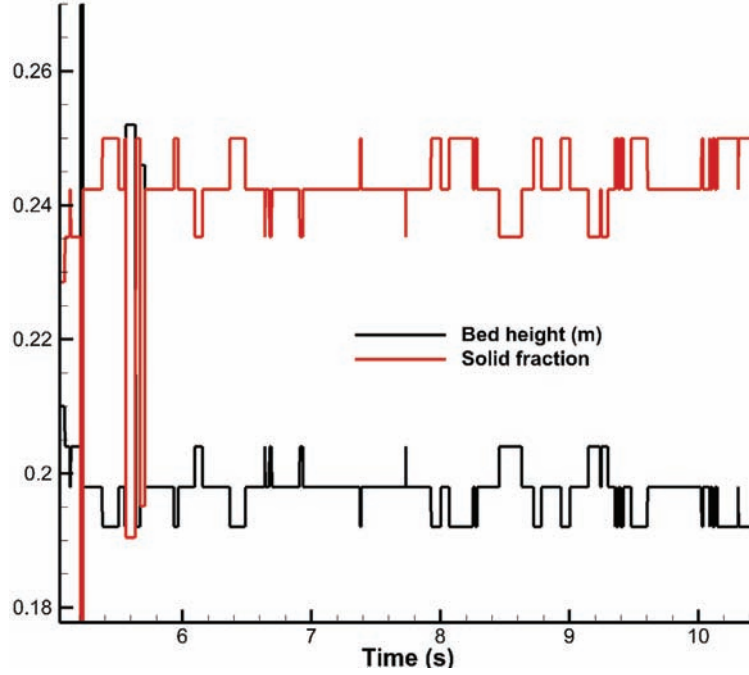
Fig. 23. Time evolution of the bed height and corresponding solid fraction over time.
