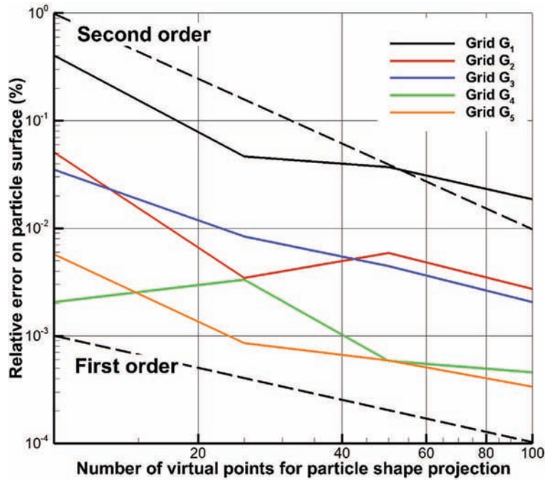
Fig. 6. Error on the projected surface of a circular shape particle according to the number of virtual points in each space direction and to the Eulerian grid used.
