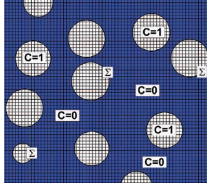
Fig. 1. Definition sketch of the fictitious domain approach for a finite size particulate flow. The underlying grid, the phase function C and the fluid-particle interface \Sigma are plotted.
