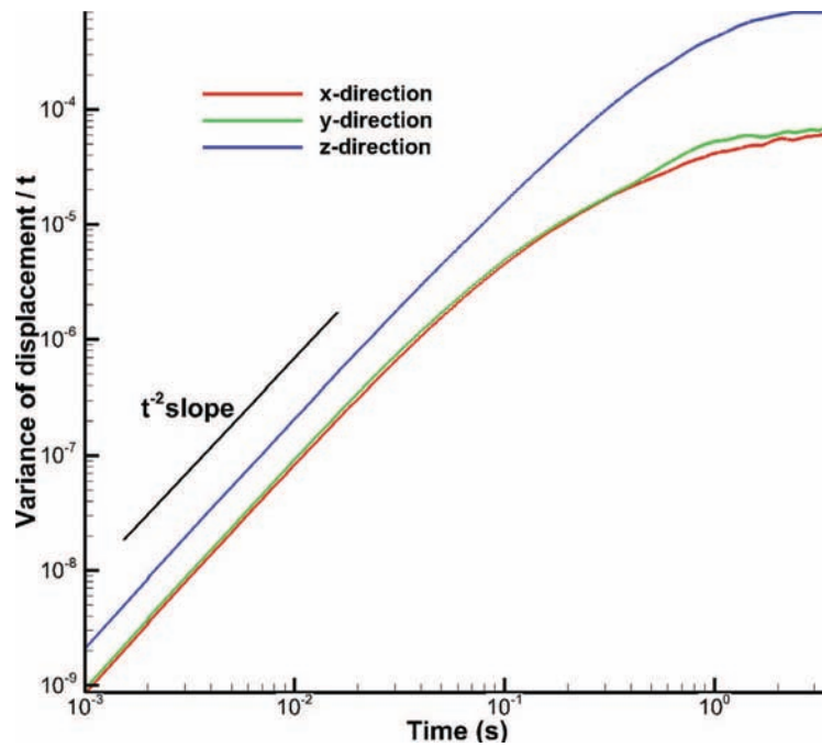
Fig. 26. Variance of the displacement of the particles \frac{M_{aa}}{t} according to time.
