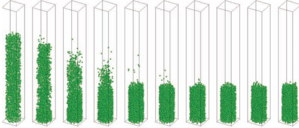
Fig. 22. Three-dimensional view of the particles inside the fluidized bed – from left to right, t = 1, 2, 3, 4, 5, 6, 7, 8, 9 and 10 s.
