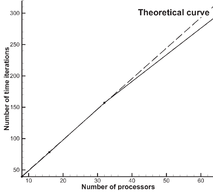
Fig. 12. Evolution of the time iterations calculated in one hour of CPU time according to the number of processors.
