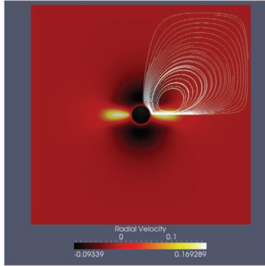
Fig. 15. Radial velocity magnitudes and streamlines in a slice for the case \mu = 10^{-2} Pa.s.
