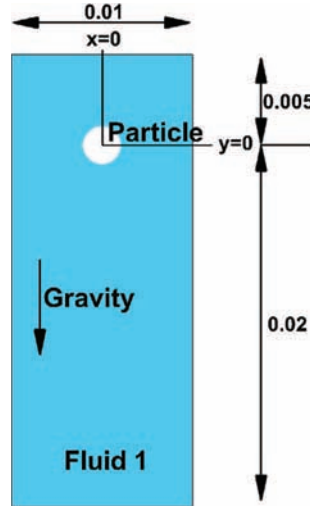
Fig. 9. Definition sketch of the settling of a cylindrical shape particle.
