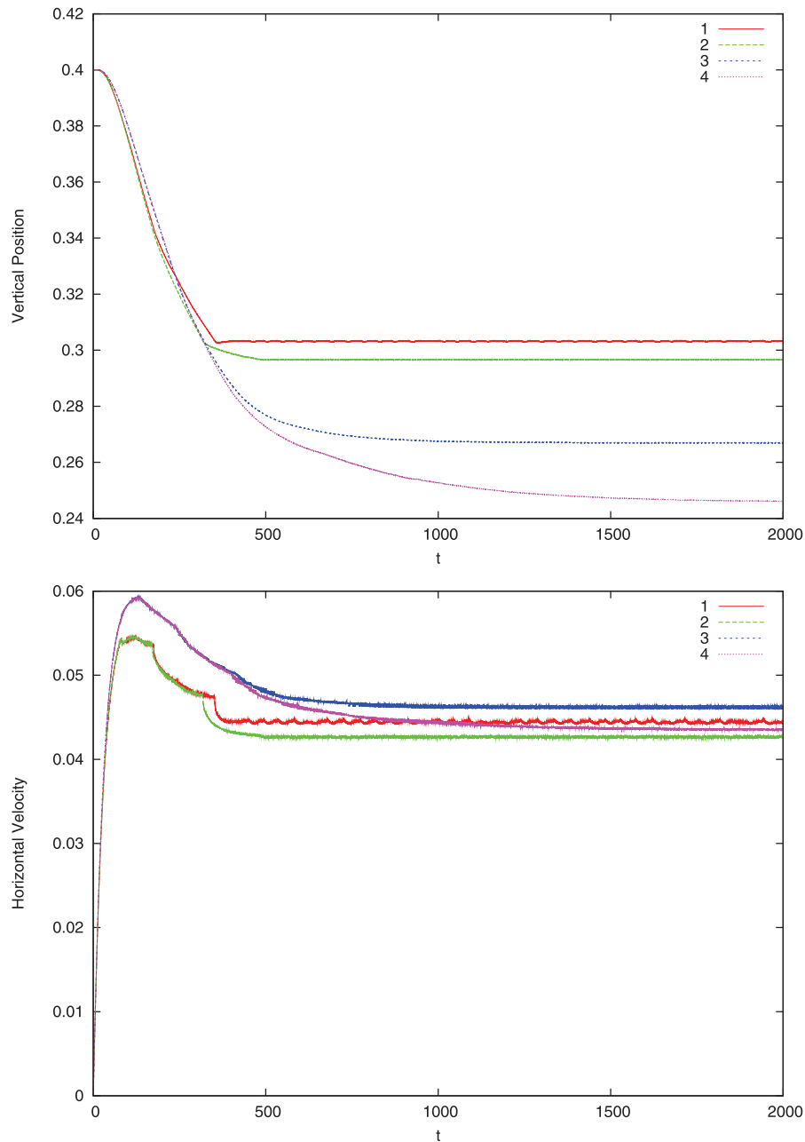
Fig. 19. Time evolution of the vertical position (top) and horizontal velocity component (bottom) of the particle for viscous laws NVL1 (red line), NVL2 (green line), NVL3 (blue line) and NVL4 (pink line). (For interpretation of the references to color in this figure, the reader is referred to the web version of this article.)
