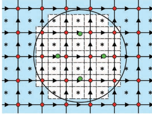
Fig. 3. Position in two dimensions of the reference Lagrangian points (green points) used to interpolate the Lagrangian velocity at the barycenter of the particles. (For interpretation of the references to color in this figure, the reader is referred to the web version of this article.)
