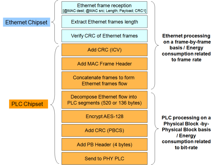
Fig. 1. Processing of an Ethernet frame through the PLC modem
