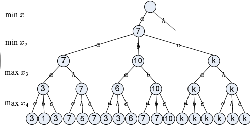
Fig. 2. Labeling Tree for Example 1
