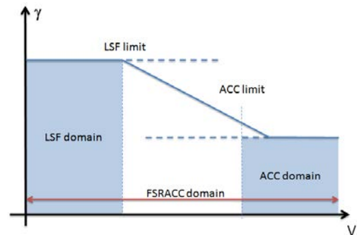
Fig. 3. Operating area of an longitudinal ADAS : Low Speed Following (LSF), Adaptive Cruise Control (ACC) and Full Speed Range ACC (FSRACC)
