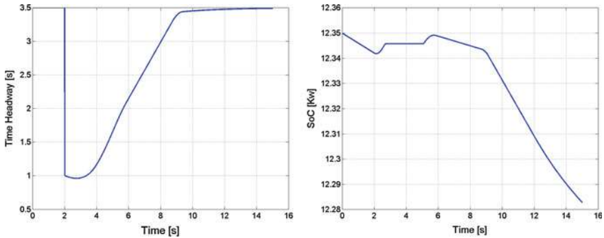
Fig. 7 Evolution of the time headway and the SoC during a cut in use case
