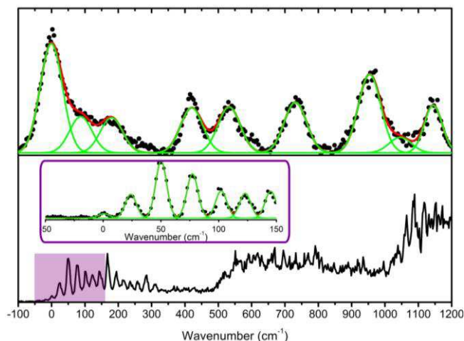
Figure 2: Low energy part of the spectra of the C_2H^+ (a) and C_2Ag^+ (b) complexes. In panel (b) the inset shows an amplification with better resolution of the first 150\text{ cm}^{-1} of the spectrum of the C_2Ag^+ complex, in which a low vibrational frequency progression composed of narrow bands is observed. The vibrational bands were fitted to Voigt profiles.
