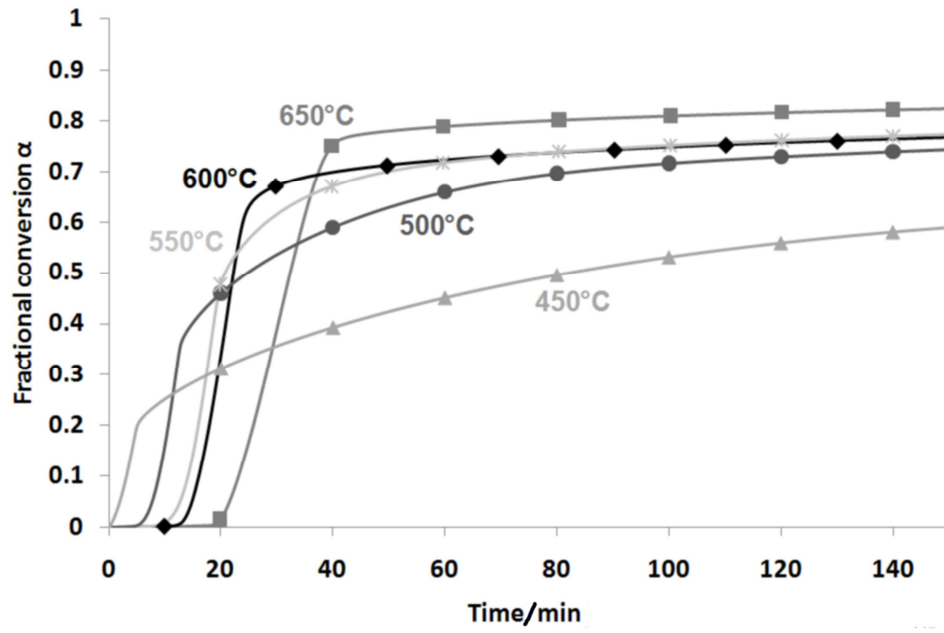
Figure 1: Isothermal and isobaric kinetic curves of CaO carbonation under a \text{CO}_2 partial pressure of 5 kPa.
