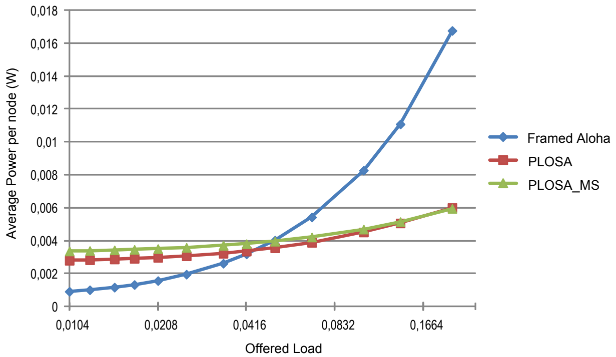
Figure 5: Average power per node.
