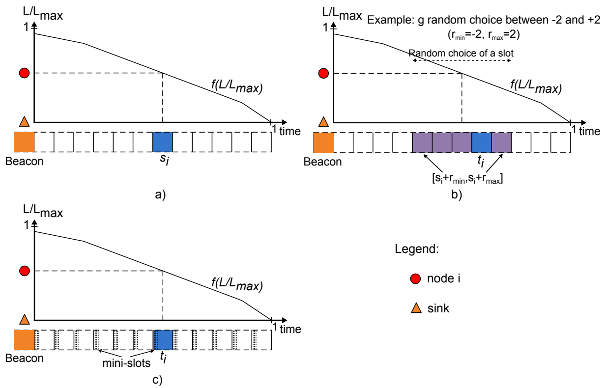
Figure 1: Transmission window mechanisms. a) Main principle. b) Random slot selection. c) Mini-slot selection.
