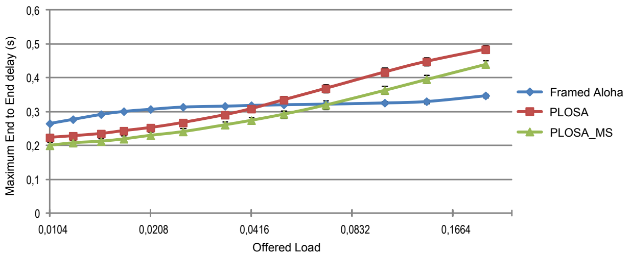
Figure 8: Maximum End-to-End delay.
