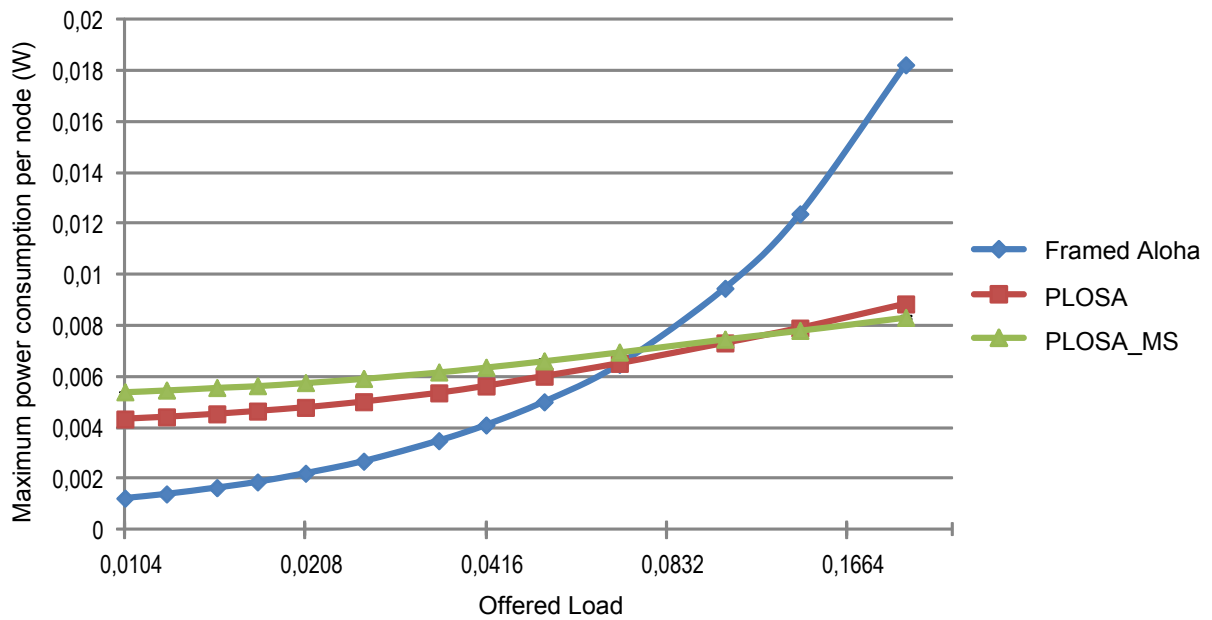
Figure 6: Maximum energy consumption.
