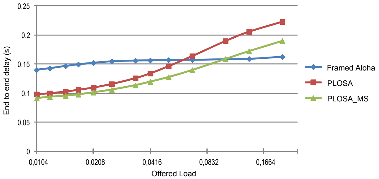
Figure 7: Average End-to-End delay.
