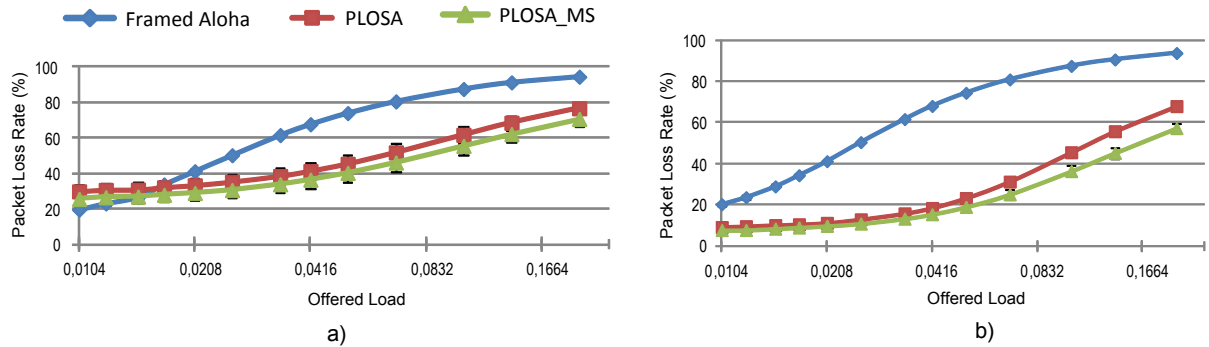
Figure 4: Packet Loss Rate under different topologies and densities. a) 80-node random topology. b) 160-node random topology.
