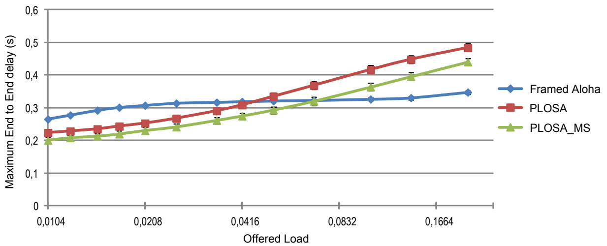
Figure 8: Maximum End-to-End delay.
