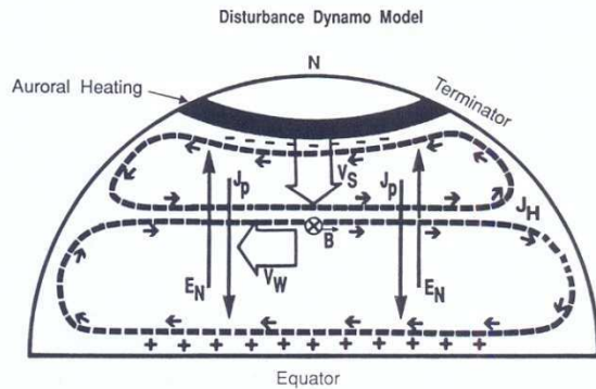
Figure 9 Schematic of the variables in the Blanc-Richmond (1980) theory. The Joule heating from the storm is assumed to extend uniformly around a high-latitude zone. The southward meridional winds at F region heights arising from this heating is shown as the arrow V_s . Due to the action of the Coriolis force, the southward meridional wind produces westward zonal motion (shown as the arrow V_w ). The zonal motion of the ions in combination with the downward component of the magnetic field (shown as \otimes \mathbf{B} ) produces an equatorward Pedersen current (shown as J_p ). The Pedersen current builds up positive charges at the equator until an electric field is established in the poleward direction opposing the flow of the Pedersen current. This poleward electric field is shown as E_N . This electric field which is perpendicular to the downward component of \mathbf{B} gives rise to an eastward Hall current with maximum intensity in middle latitudes. This Hall current is marked as J_H . The Hall current is interrupted at the terminators and gives rise to two current vortices as shown. The lower latitude disturbance current vortex is opposite in direction to the normal Sq current vortex.
