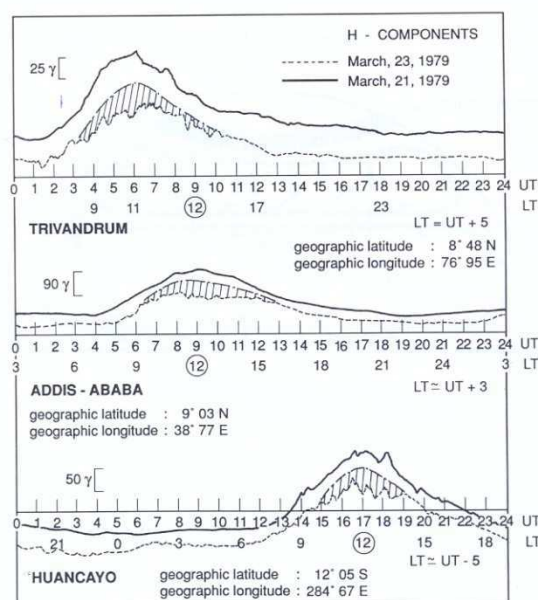
Figure 6 Trivandrum, Addis Ababa and Huancayo magnetograms (for March 21 (full line) and March 23 (dashed line), 1979. The dotted line is obtained by subtracting the difference in Dst of 36 nT (Fig. 7) between these two days. The hatched area is identified as the disturbance of ionospheric origin. (Note that Addis Ababa is not included in the calculation of Dst published in Solar Geophysical Data .)
