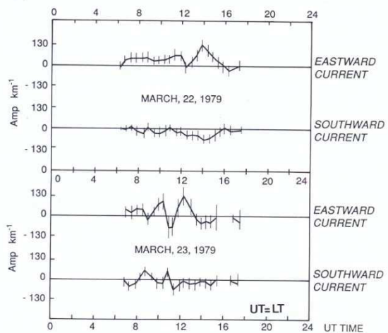
Figure 5 Height-integrated ionospheric currents over Saint-Santin on March 22 and March 23, 1979. Notice that there are strong eastward currents on both days.
