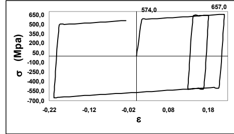
Figure 6. Uniaxial plasticity law for reinforcement bars.
