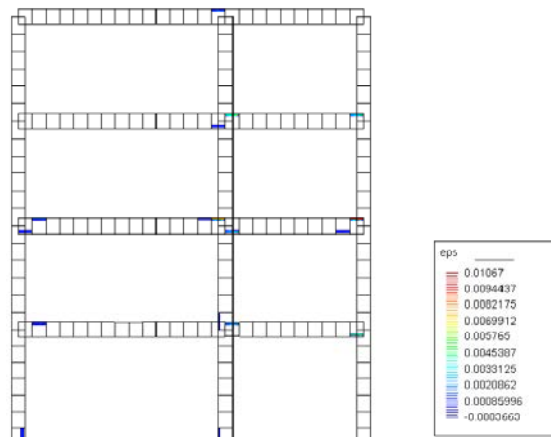
Figure 19. Position of yielded reinforcement bars at the end of the High-Level pseudodynamic test.
