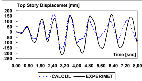
Figure 16. High -Level pseudodynamic test: top displacement versus time.
