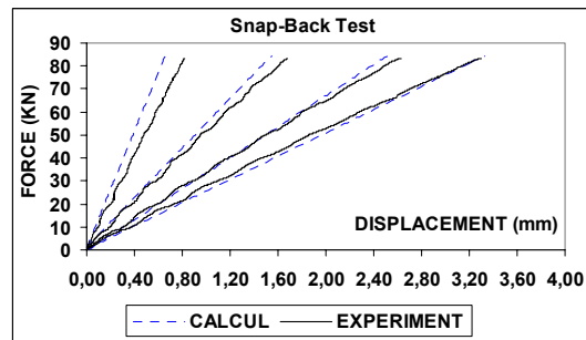
Figure 11. Simulation of the second Snap-Back test (loading applied at the top of the structure).
