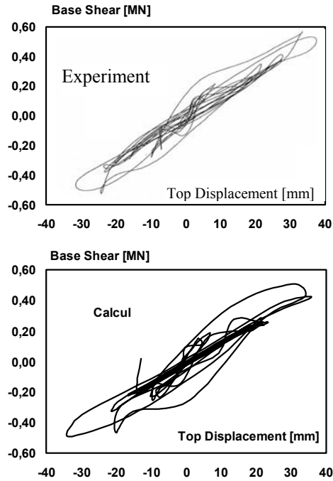
Figure 14. Low-Level pseudodynamic test: base-shear versus top-story displacement diagrams.
