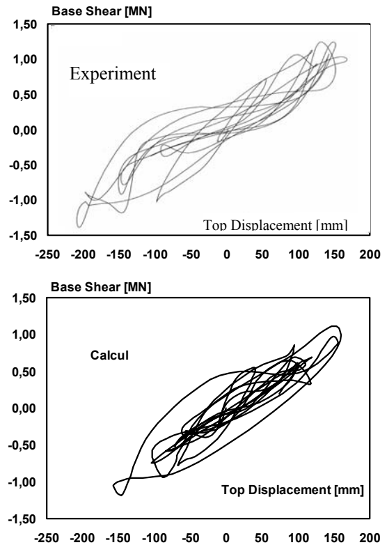
Figure 18. High-Level pseudodynamic test: base-shear versus top-story displacement diagram.
