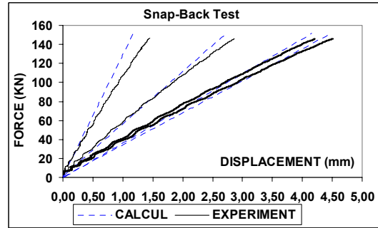
Figure 10. Simulation of the first Snap-Back test (loading applied at the third story).
