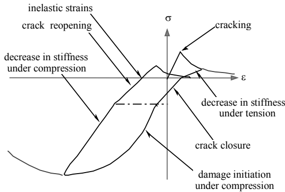
Figure 5. Uniaxial damage model for concrete.
