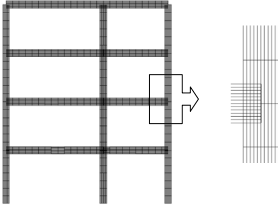
Figure 9. Mesh of the structure with multi-layer beams
