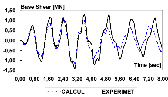
Figure 17. High -Level pseudodynamic test: Time history of the base shear.
