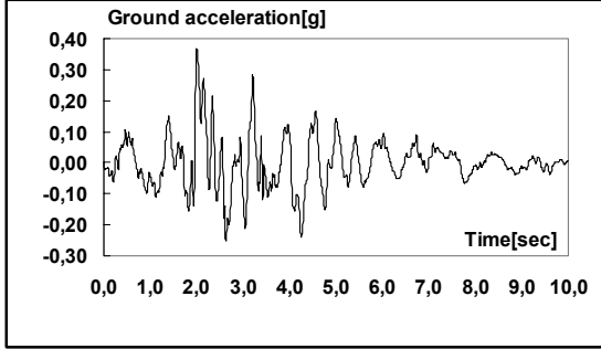
Figure 3. Friuli-like generated accelerogram.
