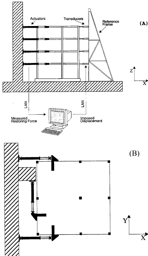
Figure 4. Experimental setup A) Side view B) plane view
