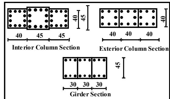
Figure 8. Section of columns and beams of the equivalent RC frame.
