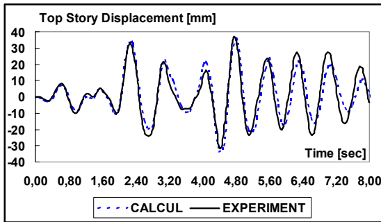
Figure 12. Low-Level pseudodynamic test: top displacement versus time.
