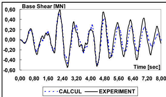
Figure 13. Low-Level pseudodynamic test: base shear versus time.
