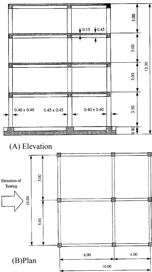
Figure 2. Layout of the specimen; (A) Elevation, (B) Plan
