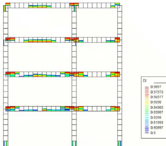
Figure 15. Damage pattern at the end of the Low-Level pseudodynamic test.
