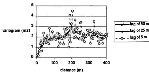
Figure 3 : Variogram from sand gravel 1 layer
