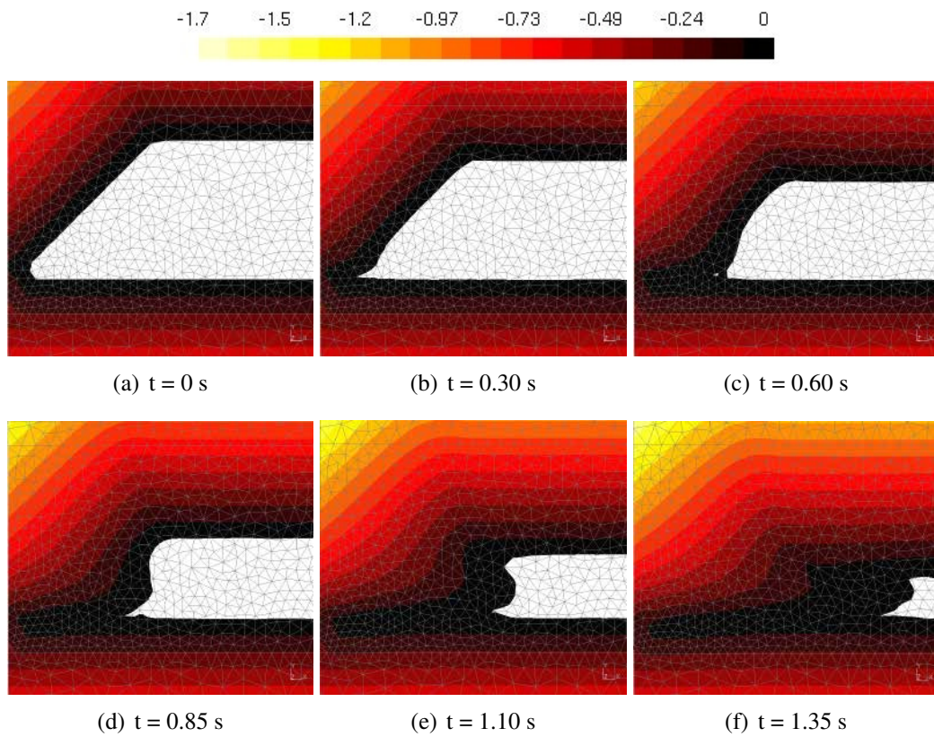
Figure 5: Evolution of the LevelSet. Negative part only.
