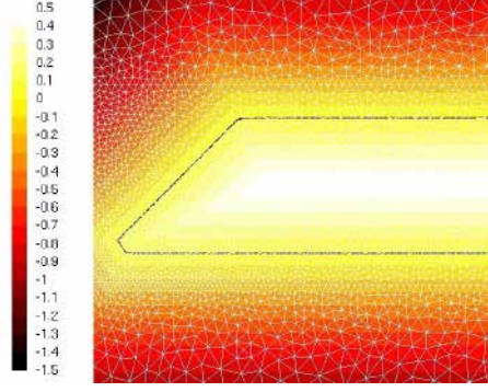
Figure 3: Initial Level Set. The iso-zero is in black.
