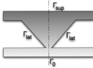
Figure 2: Geometry of the initial energy director.
