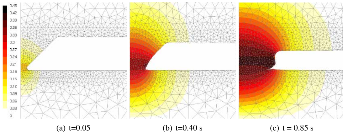
Figure 6: Temperature Field.
