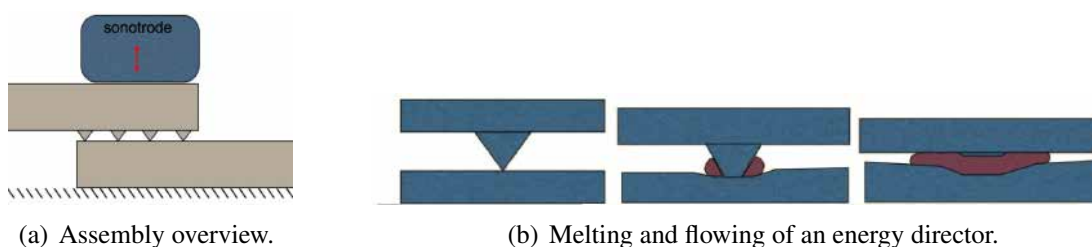
Figure 1: Ultrasonic welding of two plates
