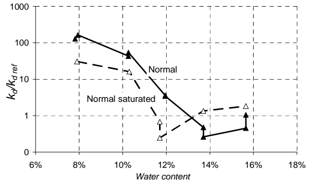
Figure 6 Relative variation of the erosion coefficient k_d for the P3 soil according to the water content at compaction.
