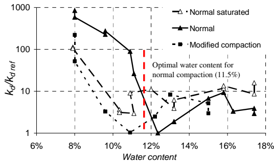
Figure 4 Relative variation of the erosion coefficient k_d for the P2 soil according to the water content at compaction.
