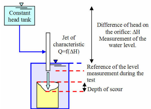
Figure 1 Schematic view of the JET.
