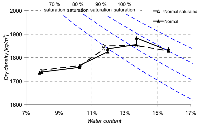
Figure 3 Dry density versus water content at compaction for the P3 soil.
