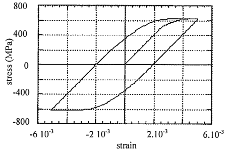
Figure 3. 1D steel constitutive law.
