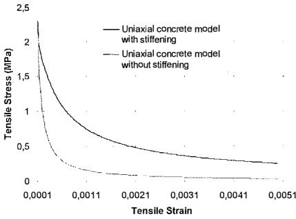
Figure 6. Taking into account the “stiffening” phenomenon.
