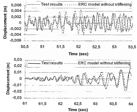
Figure 12. NUPEC - Displacement history analysis for the last loading sequences without taking into account the “tension stiffening phenomenon”.
