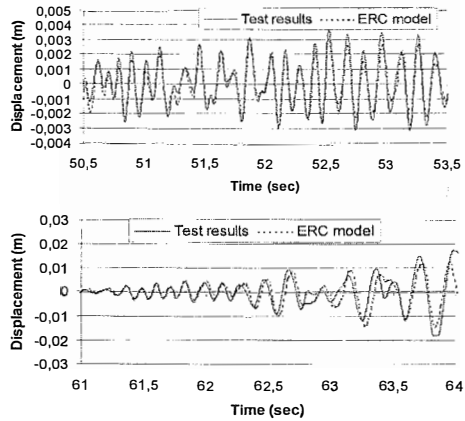
Figure 11. NUPEC - Displacement history analysis for the last loading sequences.
