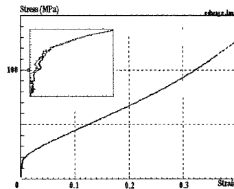
Figure 10. Quasi-static (dashed) and dynamic processing for lead
