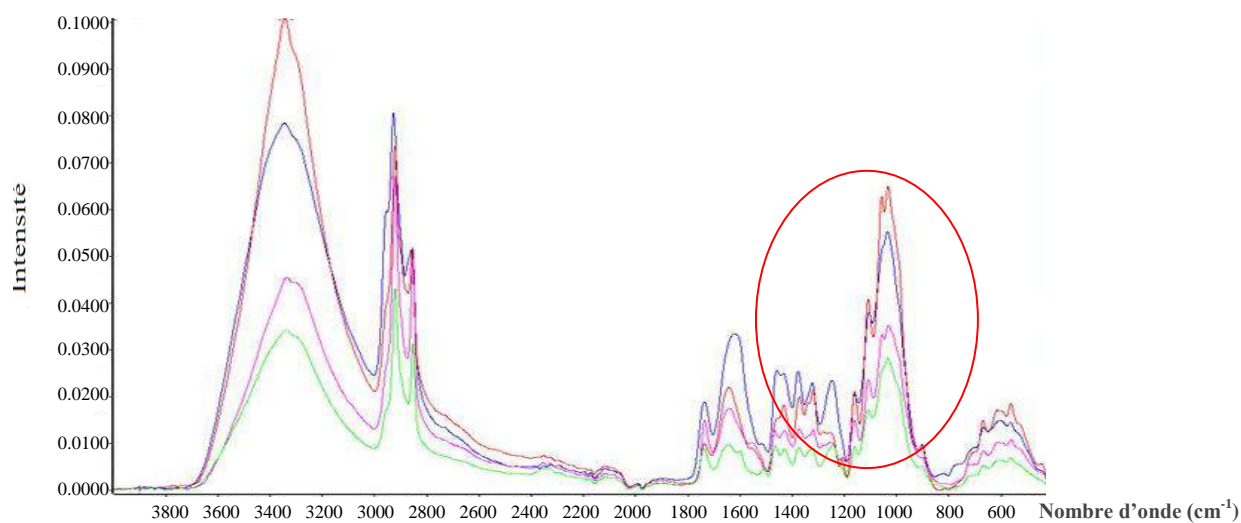
Figure 4. FTIR spectrum of -- flax, -- jute, -- hemp and -- sisal fibers
