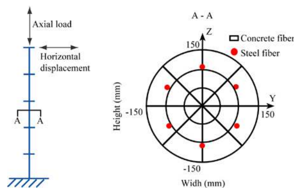
Figure 4.3. RC column under cyclic loading: Multifiber finite-element discretization.
