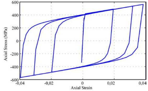
Figure 2.4. Menegotto-Pinto's cyclic model: Uniaxial stress-strain relation (isotropic hardening).
