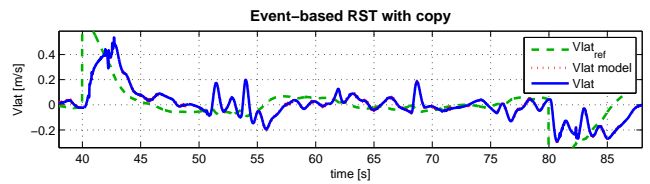
(c) Event-based RST controller.
