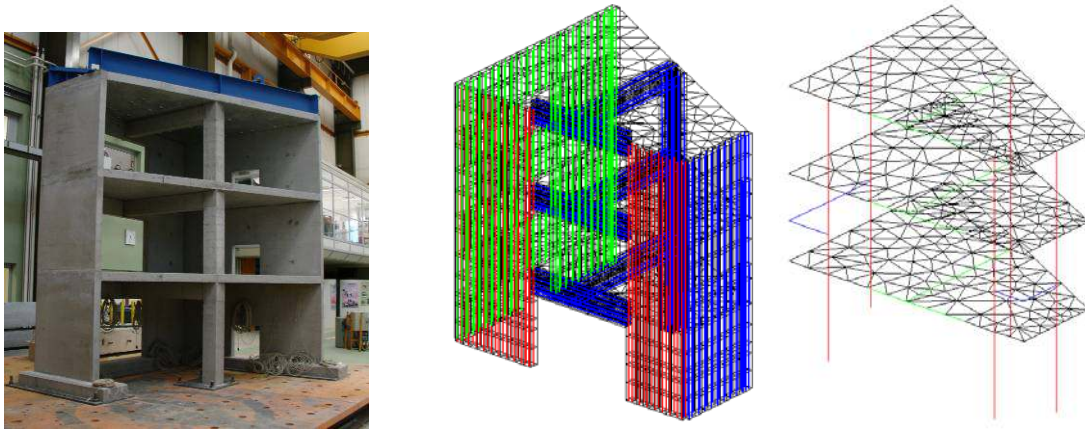
Figure 4: Photo of the SMART 2008 building and multifiber mesh
