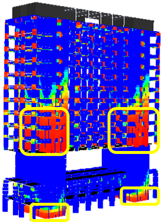
Figure 5.3. GCH (FRP design n°1) - Location of FRP sheets.
