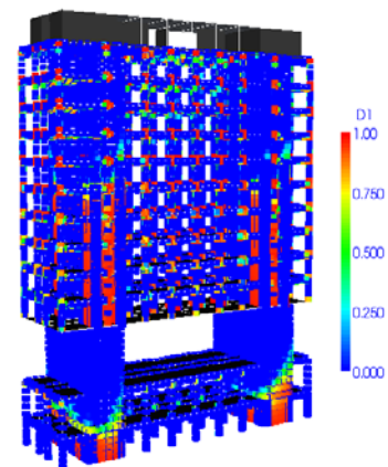
Figure 5.7. GCH (FRP optimization) – Distribution of tension damage ( DI ), final step.
