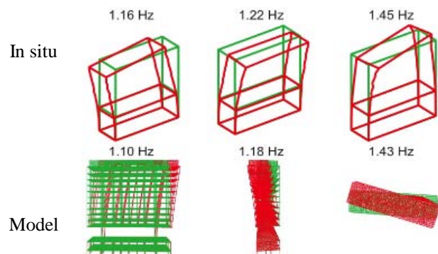
Figure 3.5. GCH – Modal analysis – In-situ records Vs model.
