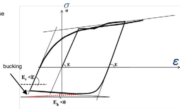
Figure 3.3. Menegotto & Pinto model - uniaxial stress-strain relation.
