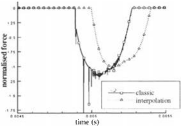
Figure 15 : Normal force
