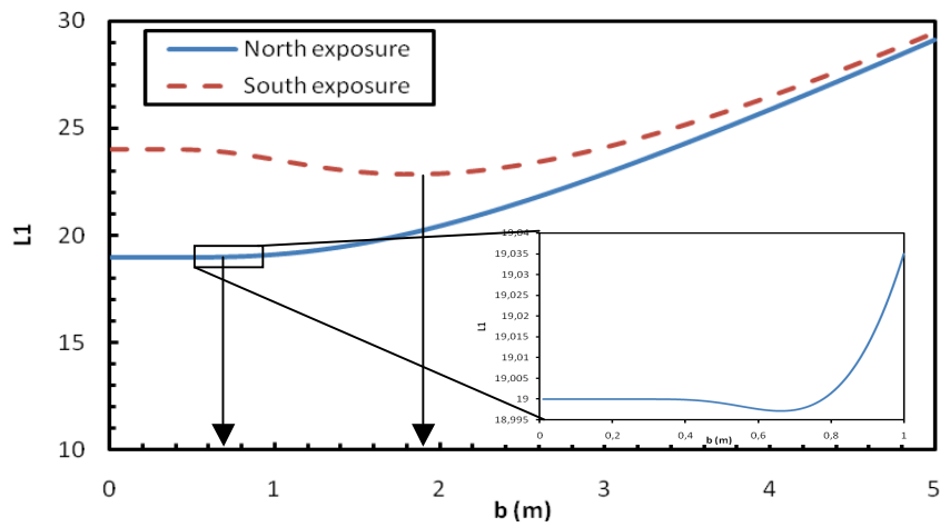
Fig 4: Evolution of function L_1 with scale of fluctuation b of C_s (Data of Bridge Ferry-Carring, Ireland)
