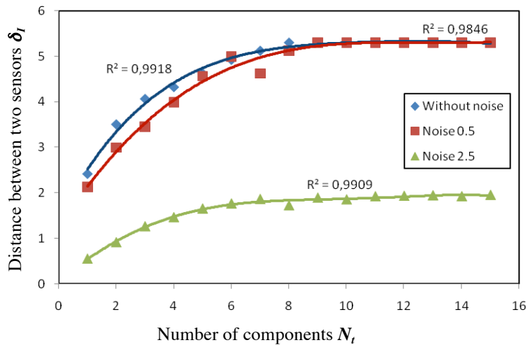
Figure 4: The curve of N_t and \delta_l considering the noise measurement satisfying P_I=90\%
