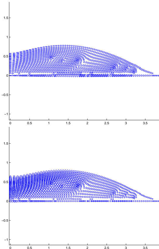
Figure 4: Orientation field for the CNT suspension at an intermediate step of the simulation (top: r - z orientation field. Bottom: r - \theta plane).
