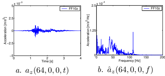
Fig. 15. (a) Time history and (b) frequency content of the free field acceleration at 64 m.
