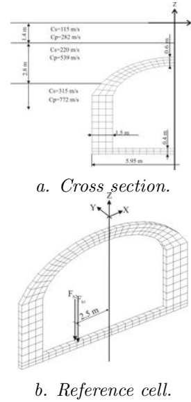
Fig. 2. (a) Cross section of the model of the metro tunnel with the soil stratigraphy and (b) finite element mesh of the reference cell and the applied forces.
