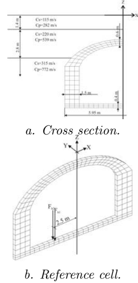
Fig. 2. (a) Cross section of the model of the metro tunnel with the soil stratigraphy and (b) finite element mesh of the reference cell and the applied forces.
