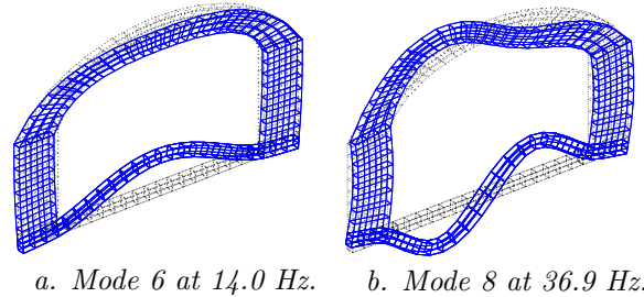
Fig. 3. Flexural modes of the reference cell of the tunnel.
