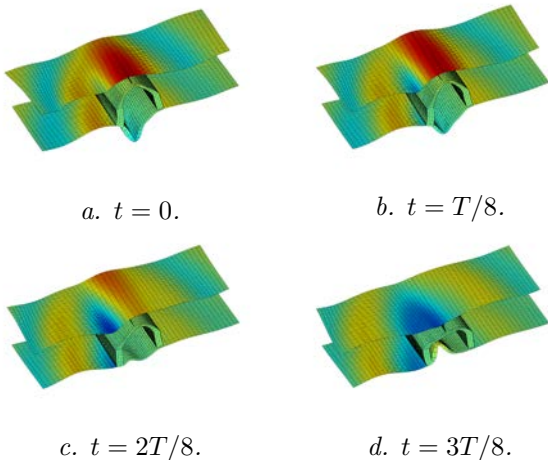
Fig. 8. Real part of the displacements of the tunnel and the soil due to a harmonic excitation on the tunnel invert at 14 Hz at (a) t = 0 , (b) t = T/8 , (c) t = 2T/8 , and (d) t = 3T/8 .
