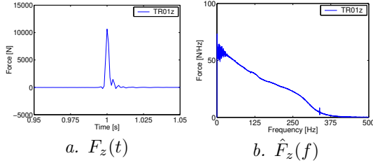
Fig. 11. (a) Time history and (b) frequency content of impact force.
