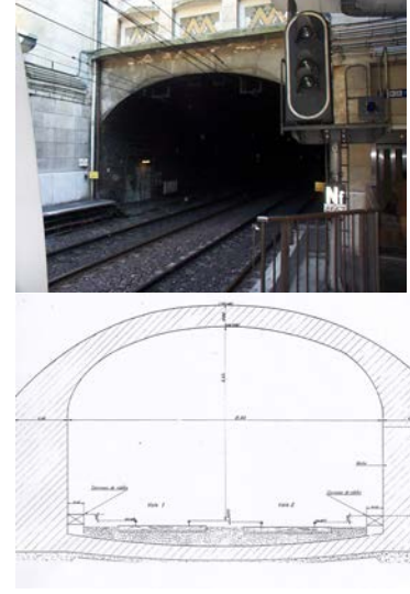
Fig. 1. Cross section of the metro tunnel on the line RER B of RATP at Cité Universitaire.
