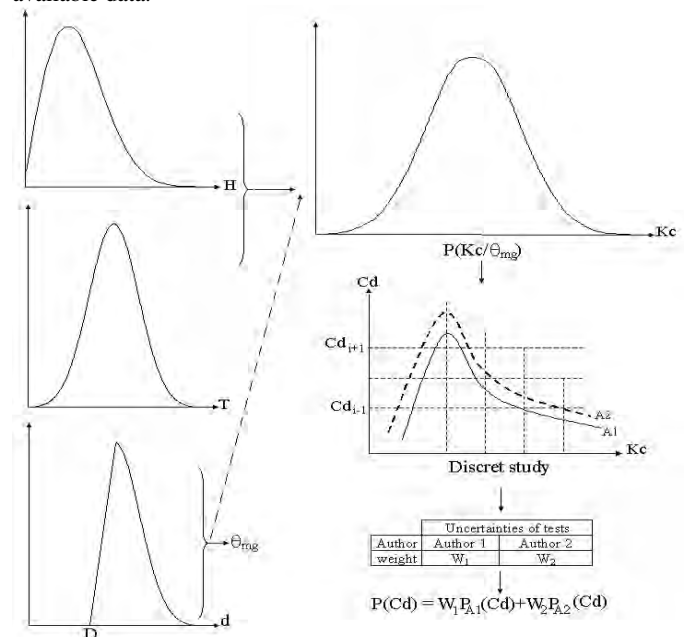
Figure 12. Plan of the probabilistic modelling of the drag coefficient.
