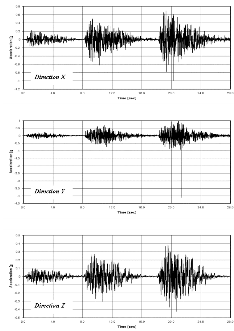
Figure 5: Chargements sismiques.
