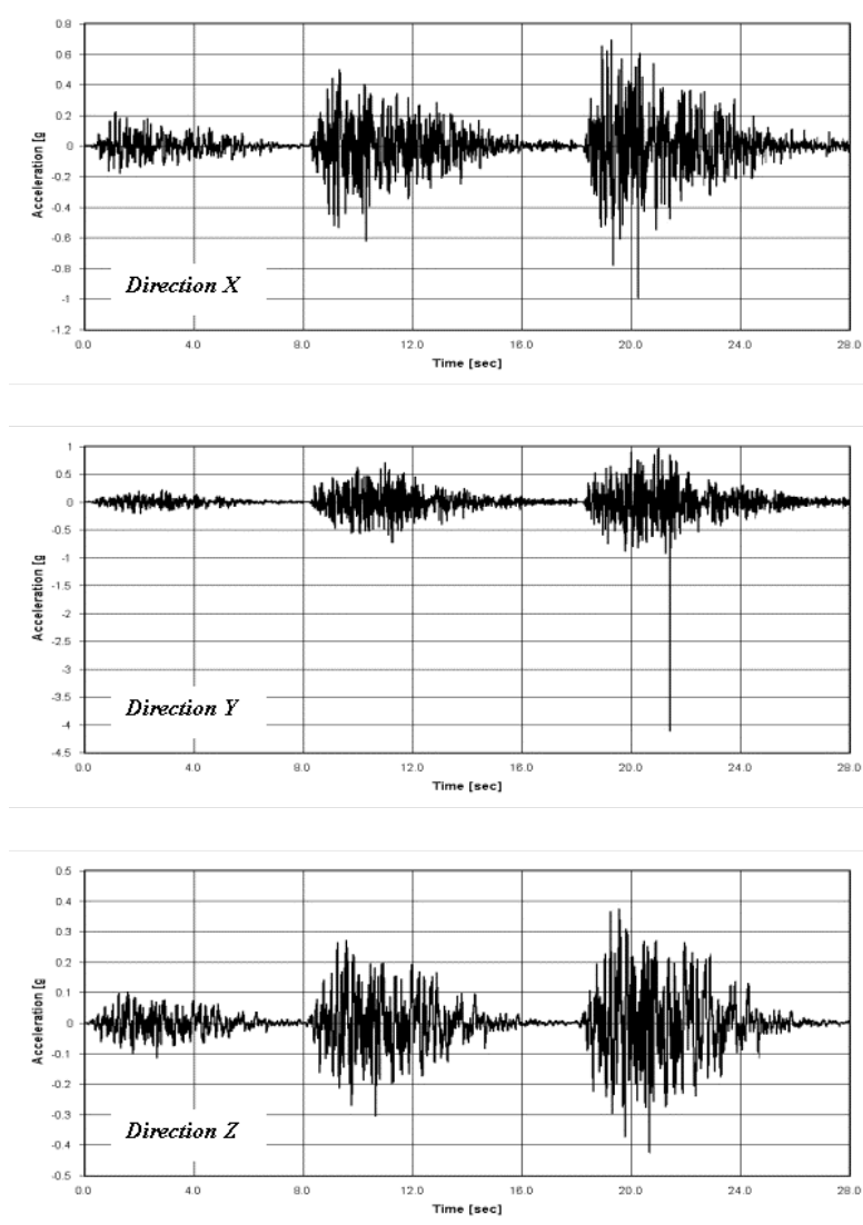
Figure 5: Chargements sismiques.
