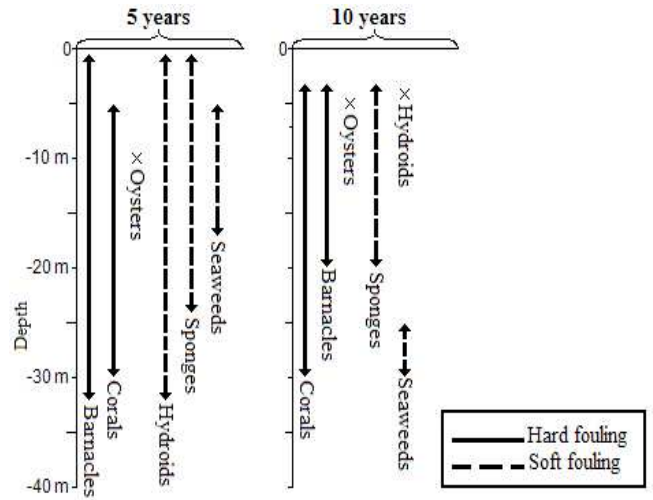
Figure 4. Distributions of fouling organisms on typical structures established in region "C".
