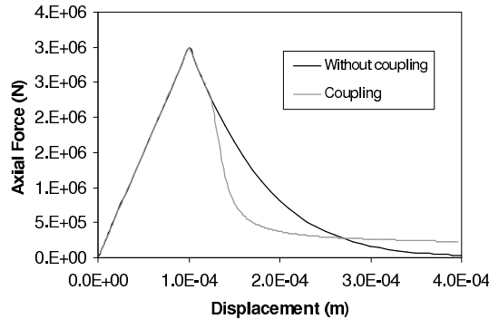
Fig. 8. 1D traction: Force - displacement curves considering or not coupling between the first and the second gradient part
