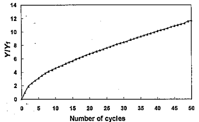
Figure 10. Normalized displacement – number of cycles relationship
