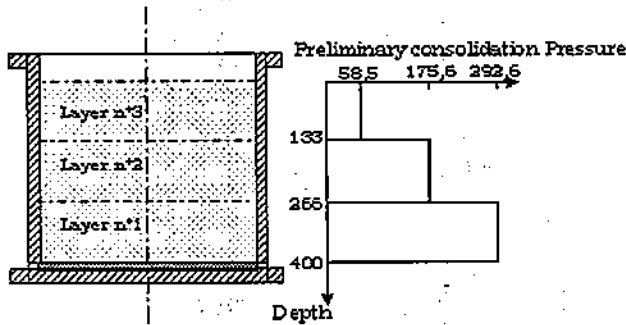
Figure 4. Preliminary consolidation pressure
