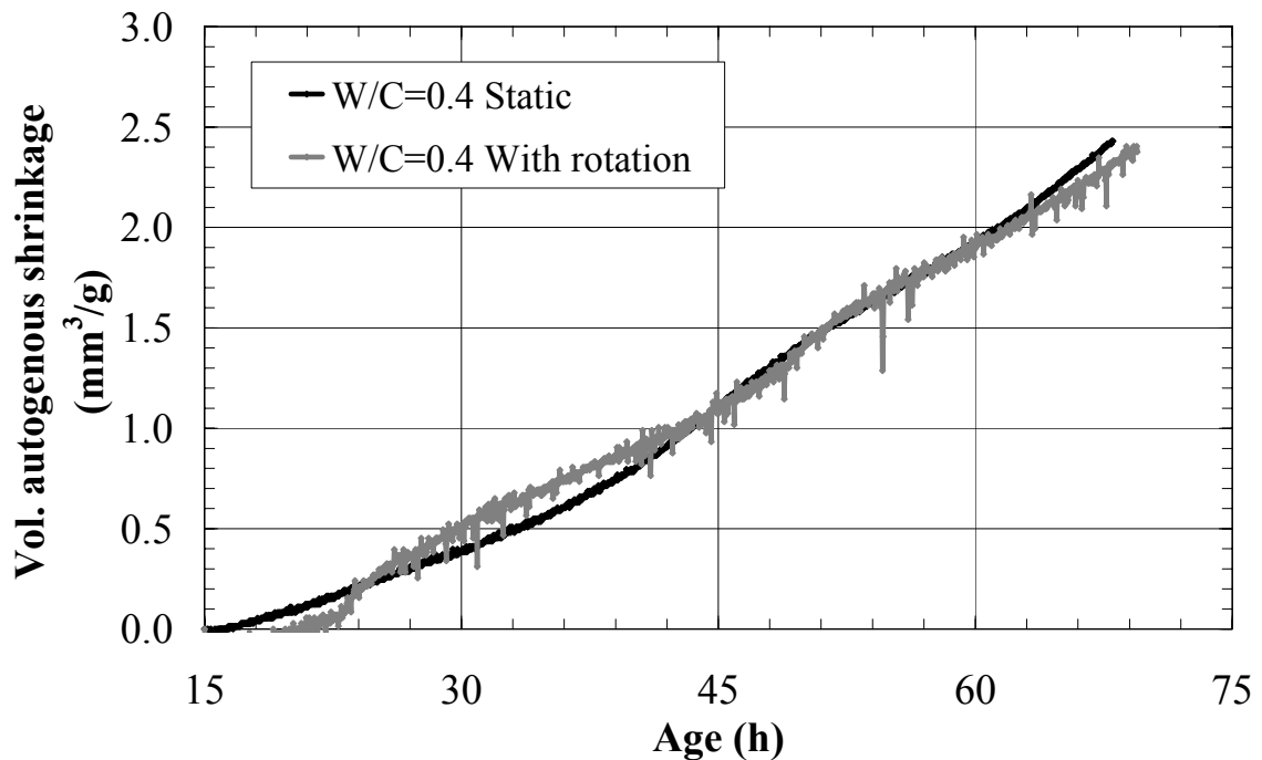
Figure 10: Volumetric autogenous shrinkage with and without rotation of the sample initialized at 15h of hydration (Cement paste with W/C=0.4 at T=20 ± 1°C)
