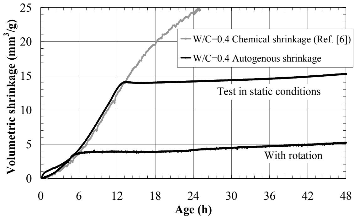
Figure 9: Comparison between chemical shrinkage and volumetric autogenous shrinkage measured with and without rotation of the sample (Cement paste with W/C=0.4 at T=20 ± 1°C)
