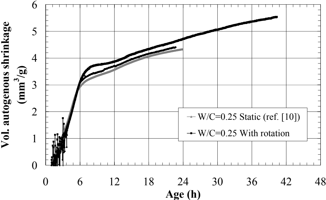
Figure 8: Volumetric autogenous shrinkage vs. hydration age (Cement paste with W/C=0.25 at T=20 ± 1°C)
