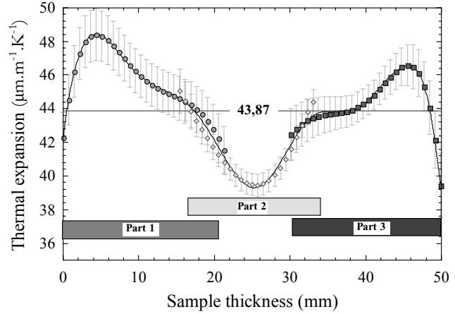
Figure 2: Experimental coefficient of thermal expansion profile of the PVC foam obtained by speckle interferometry.
