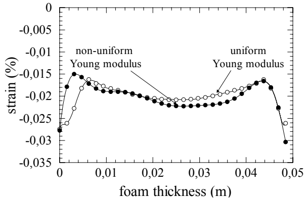
Figure 10: Comparison between the experimental strain profile and the strain simulated profile using a uniform E profile.
