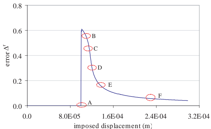
Figure 6: Evolution of the error vs loading.
