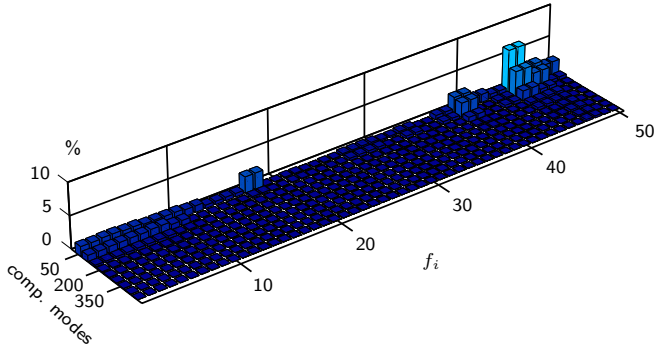
Fig. 3: Frequency deviation factors (in %) of the casing with respect to the number of component modes in the reduced model
