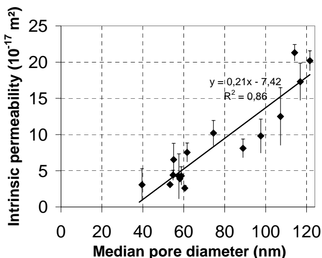
Figure 5. Intrinsic permeability.
