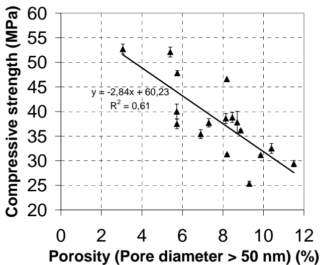
Figure 4. Compressive strength.
