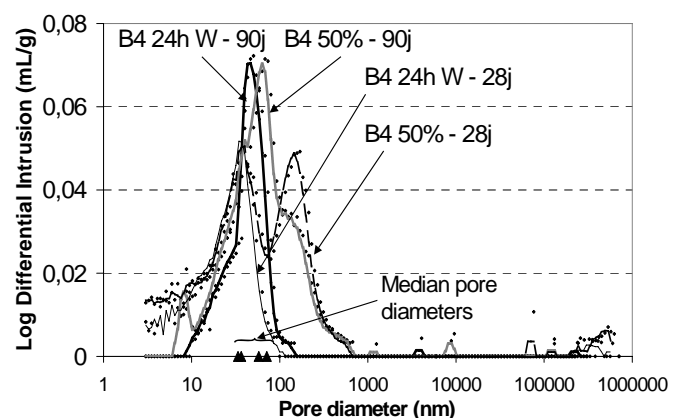
Figure 3. Pore size distribution of B4 concrete.
