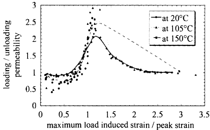
Figure 7: Loading to unloading intrinsic permeability ratio vs applied relative strain
